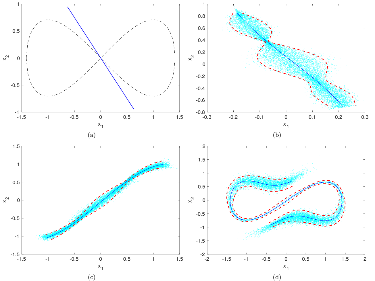
FIG. 3. Original curve (a), and subsequent advected curve points (cyan), with the deterministically advected curve (solid blue) and R_2(t) (dashed red), for the stochastic Duffing equation as described in Section IV: (b) t = 0.5 , (c) t = 2 and (d) t = 5 .
