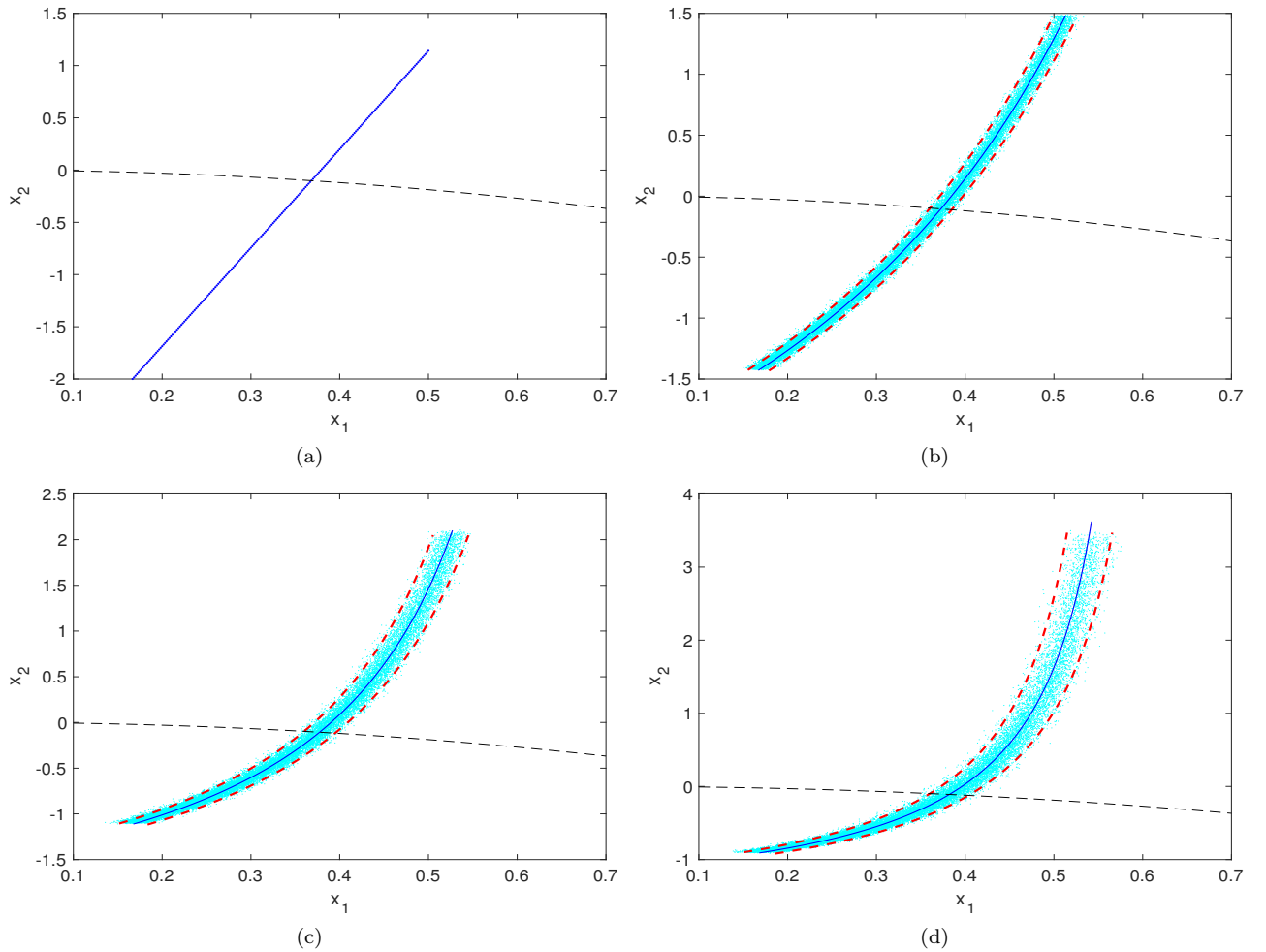
FIG. 6. Original curve (a), and subsequent advected curve points (cyan), with the deterministically advected curve (solid blue) and the theoretical zone R_2(t) (dashed red), for the flow (17) stochastically perturbed with \sigma = \text{Id} . The flow (17) is expanding above the dashed black curve. (b) t = 0.1 , (c) t = 0.2 and (d) t = 0.3 .
