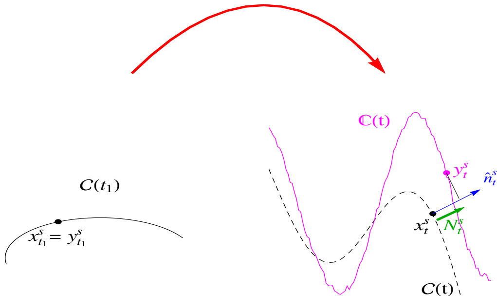
FIG. 1. The advection of \mathcal{C}(t_1) from the time t_1 (left) to the time t (right), showing the resulting deterministic curve \mathcal{C}(t) (dashed black) and a stochastic realization \mathfrak{C}(t) (solid magenta).
