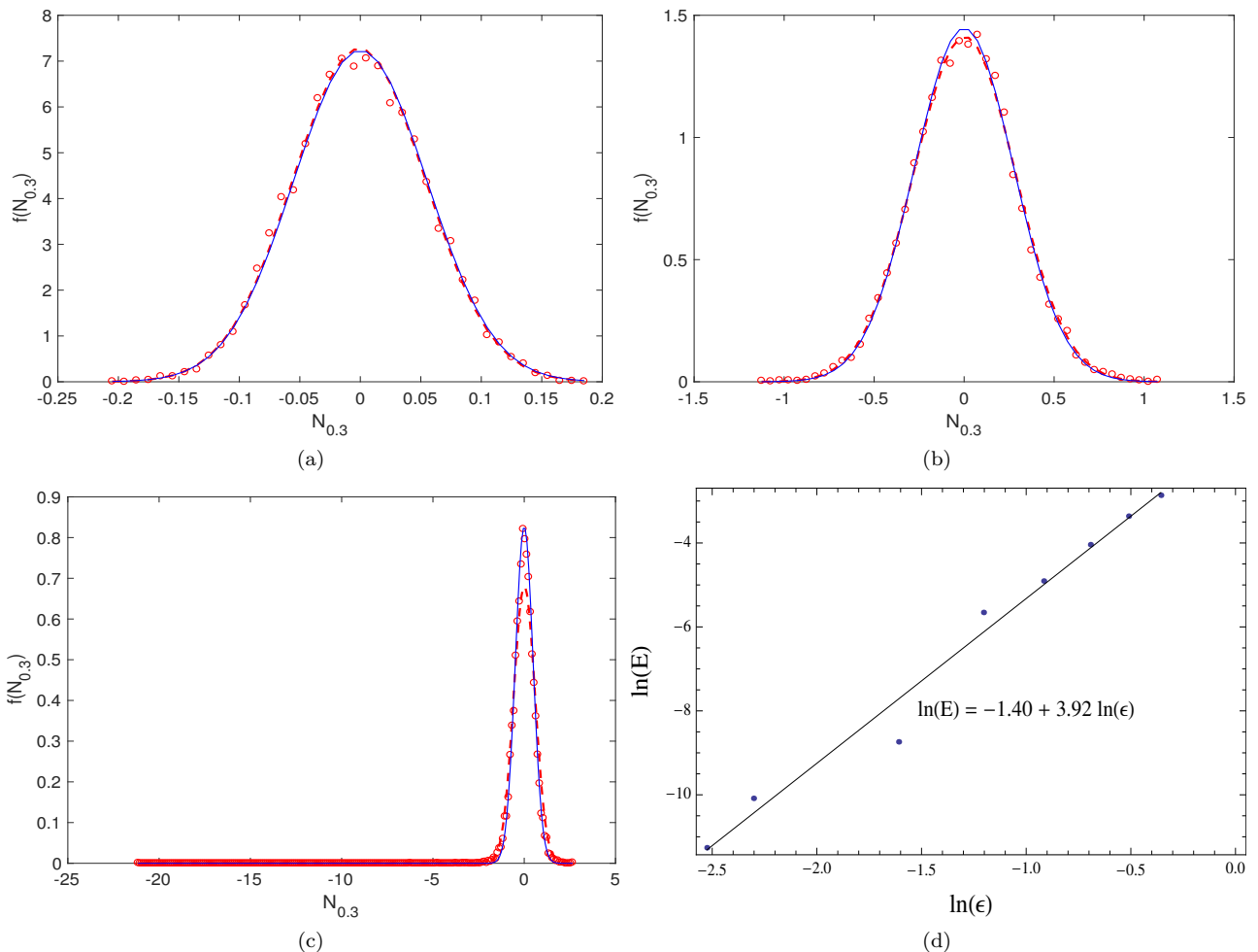
FIG. 7. A comparison of the frequency statistics f(N_{0.3}) (red circles), its imputed normal distribution (dashed red curve), and theoretical (normalized) distribution (solid blue curve) for (a) \epsilon = 0.08 , (b) \epsilon = 0.4 and (c) \epsilon = 0.7 for the compressible flow as described in the text. (d) shows the variation of the error (16) (with subscript 0.3) with \epsilon (blue dots), and a linear fit.
