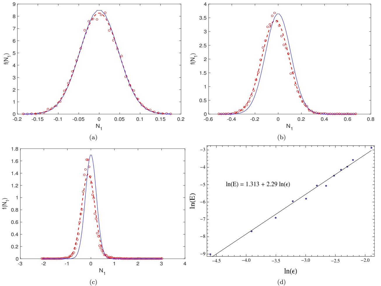
FIG. 5. A comparison between the frequency statistics f(N_1) of the numerically simulated N_1 (red circles), its imputed normal distribution (dashed red curve), and theoretical (normalized) distribution (solid blue curve) for (a) \varepsilon = 0.03 , (b) \varepsilon = 0.07 and (c) \varepsilon = 0.15 for the Duffing flow as described in the text. (d) shows the variation of the error (16) with \varepsilon (blue dots), and a linear fit.
