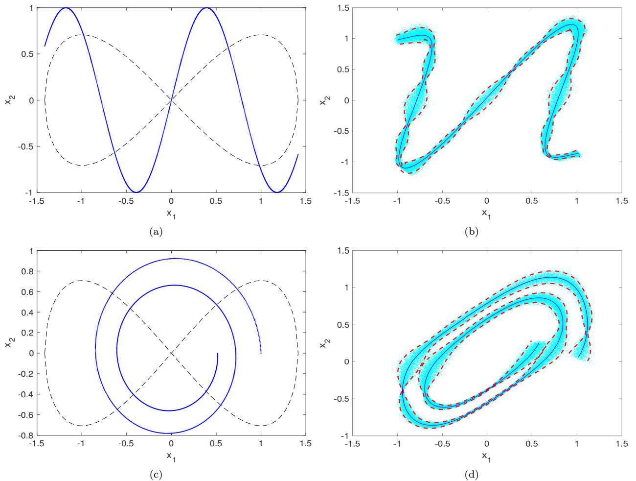
FIG. 4. Several choices of initial curves seeded with 1000 points [left panel], and their resulting stochastic advection [right panel] under the Duffing flow to time t = 0.5 .
