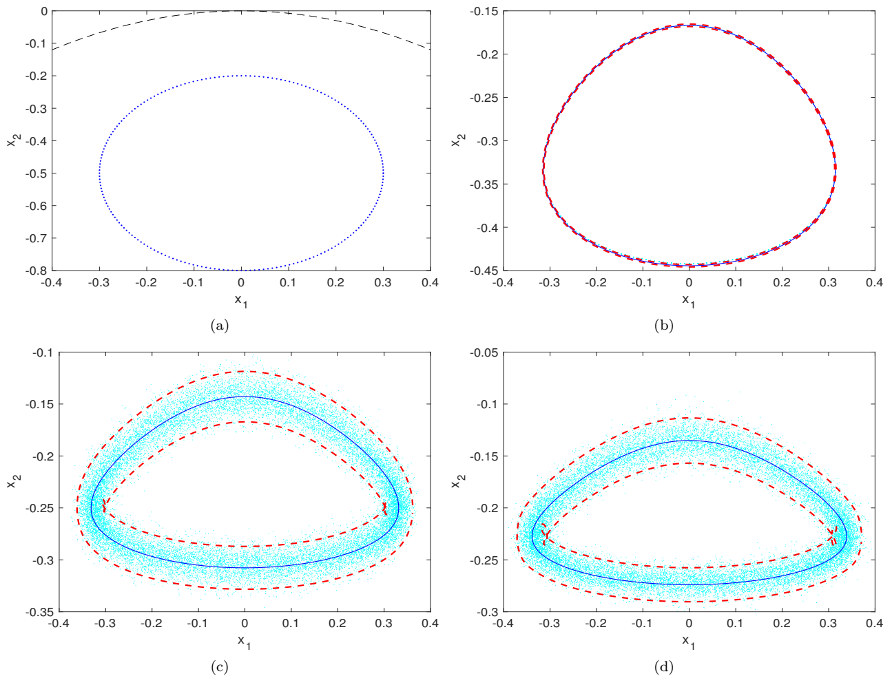
FIG. 8. Original curve (a), and subsequent advected curve points (cyan), with the deterministically advected curve (solid blue) and the theoretical region R_2(t) (dashed red), for the flow (17) stochastically perturbed with \sigma(\mathbf{x}, t) = \chi_{[0.5,1]}(t) \text{Id} : (b) t = 0.5 , (c) t = 1 and (d) t = 1.2 .
