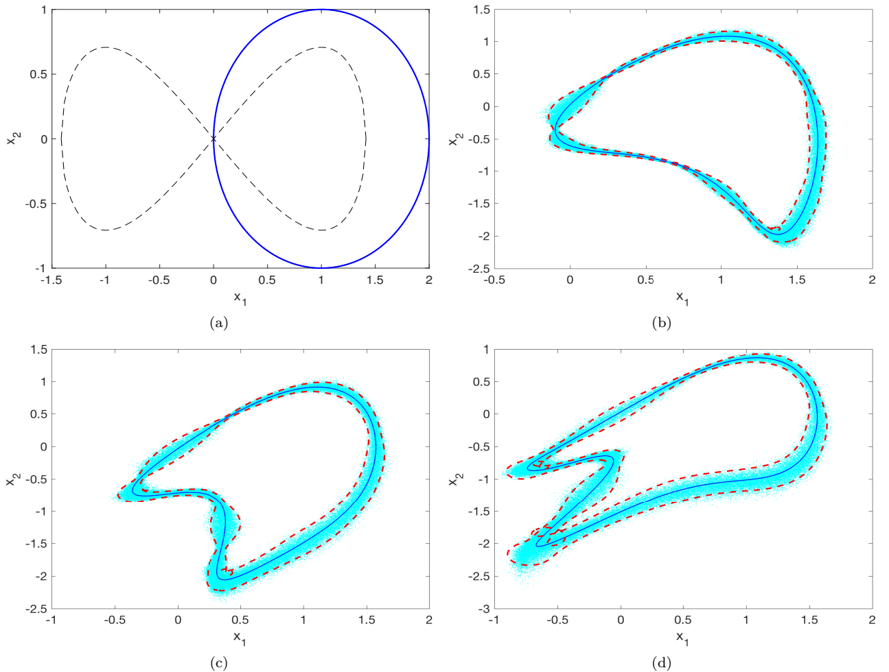
FIG. 2. Original curve (a), and subsequent advected curve points (cyan), with the deterministically advected curve (solid blue) and the theoretical R_2(t) (red dashed), for the stochastic Duffing equation as described in Section IV: (b) t = 0.5 , (c) t = 1 and (d) t = 1.5 .
